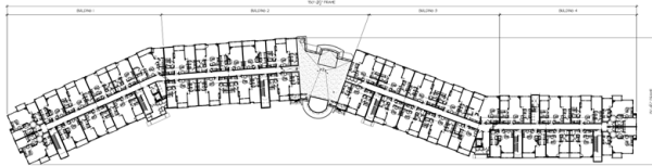
1 Third Floor Orientation Plan
